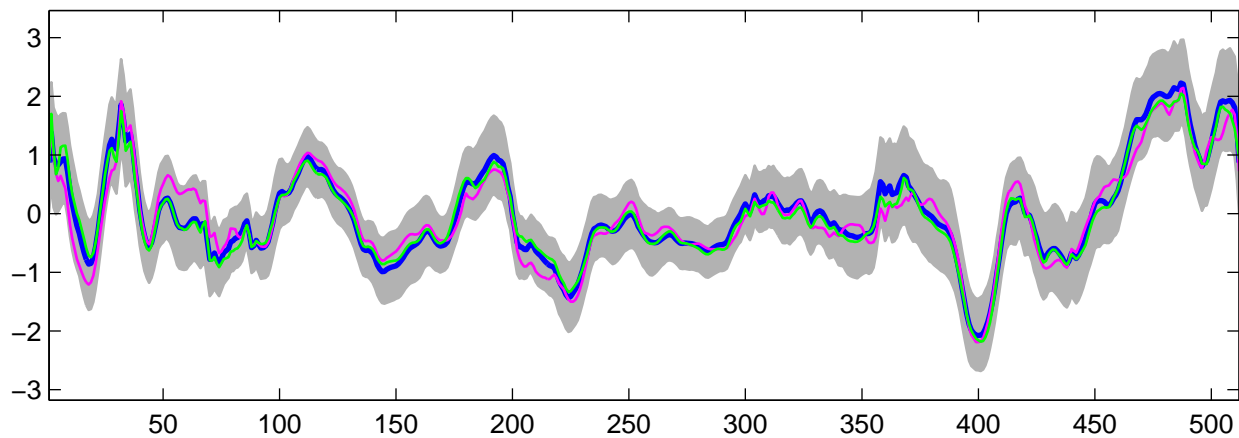
Estimated U_{\theta}(t) using G-WFMM: DE data, run 1
