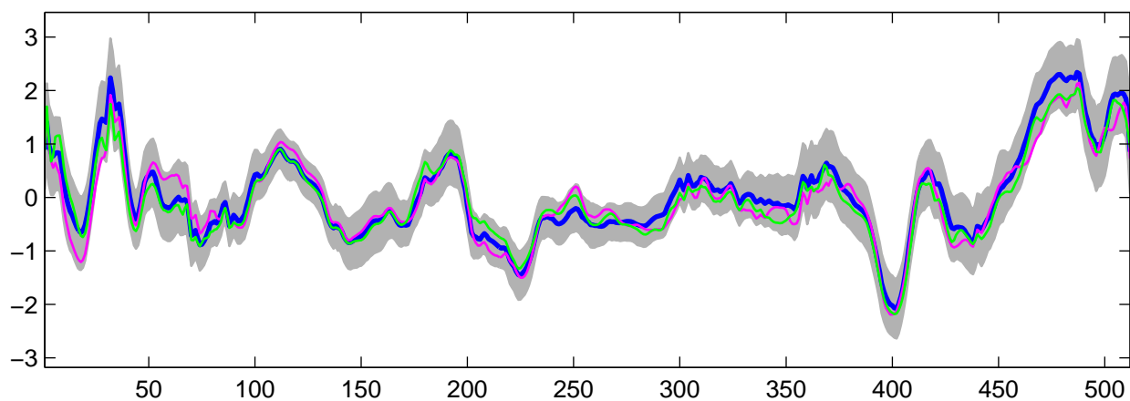
Estimated U_{\theta}(t) using R-WFMM: DE data, run 1
