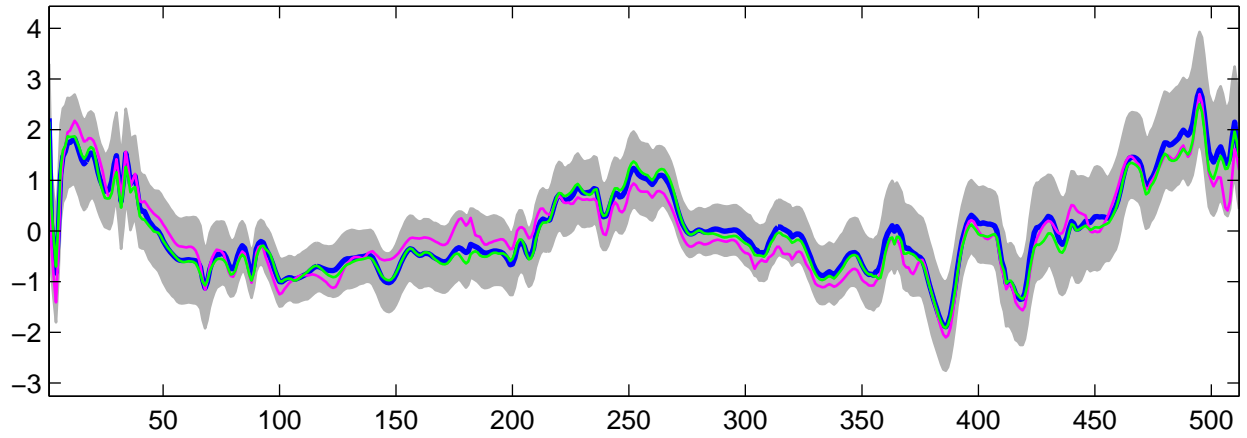
Estimated U_{\theta}(t) using G-WFMM: Normal data, run 1
