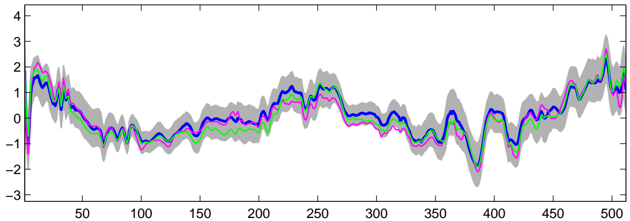
Estimated U_{\theta}(t) using R-WFMM: Normal data, run 1
