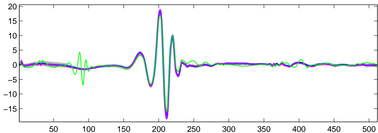
Estimated U_{\theta}(t) using R-WFMM: t_1 data, run 1
