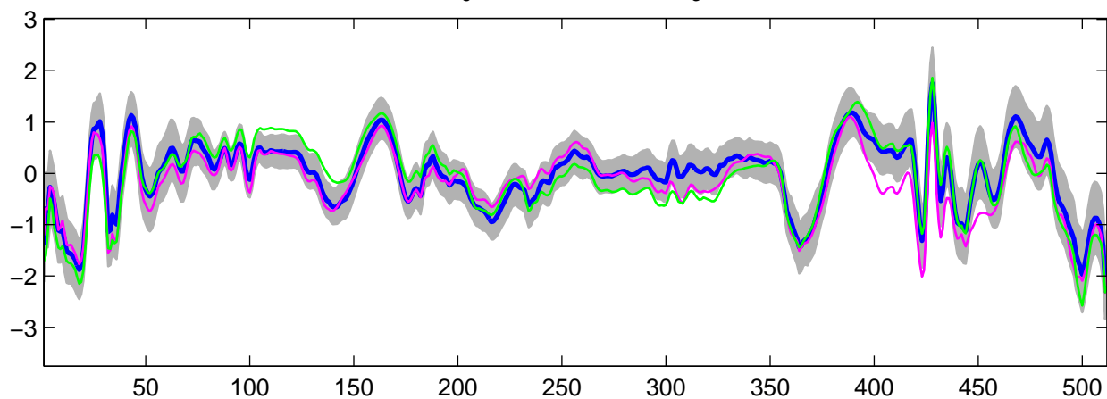
Estimated U_\theta(t) using R-WFMM: t_3 data, run 1
