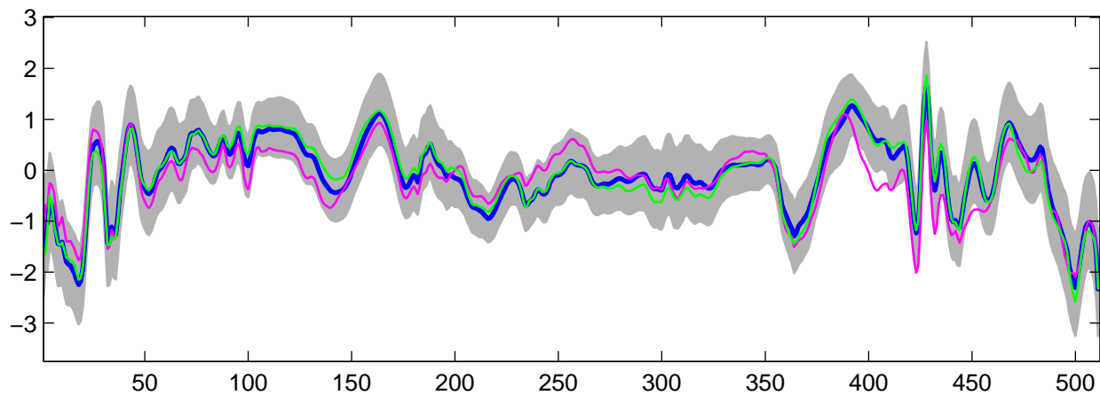
Estimated U_\theta(t) using G-WFMM: t_3 data, run 1
