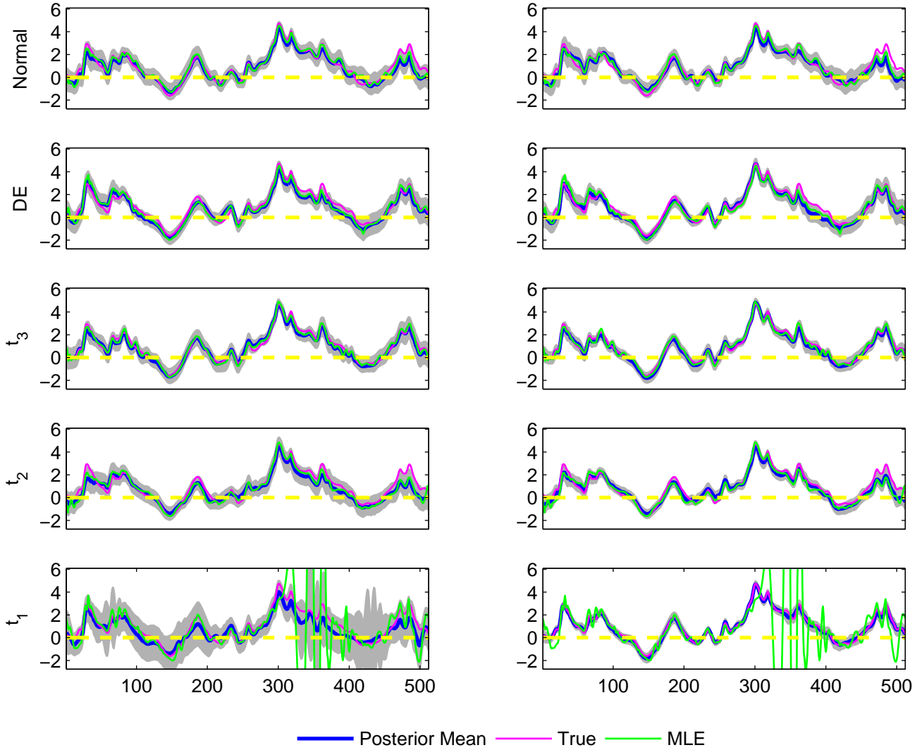
The estimated B_2(t) for 5 simulated datasets, simulation run 10
