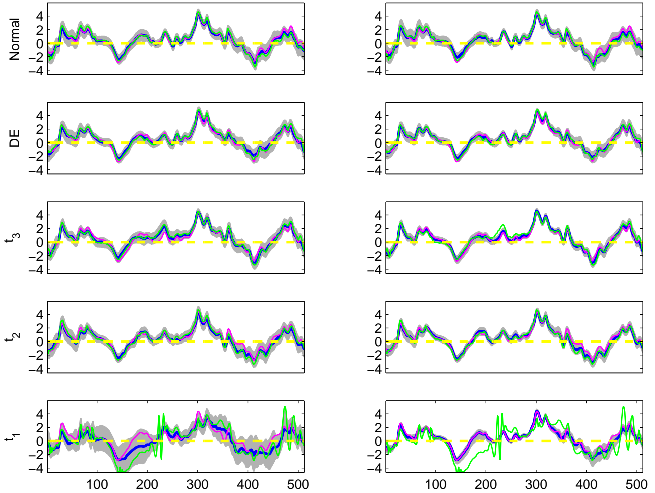
The estimated B_3(t) for 5 simulated datasets, simulation run 10 G-WFMM R-WFMM
