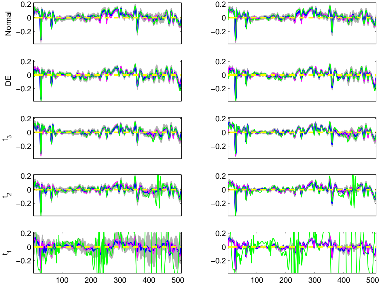
The estimated B_5(t) for 5 simulated datasets, simulation run 10
