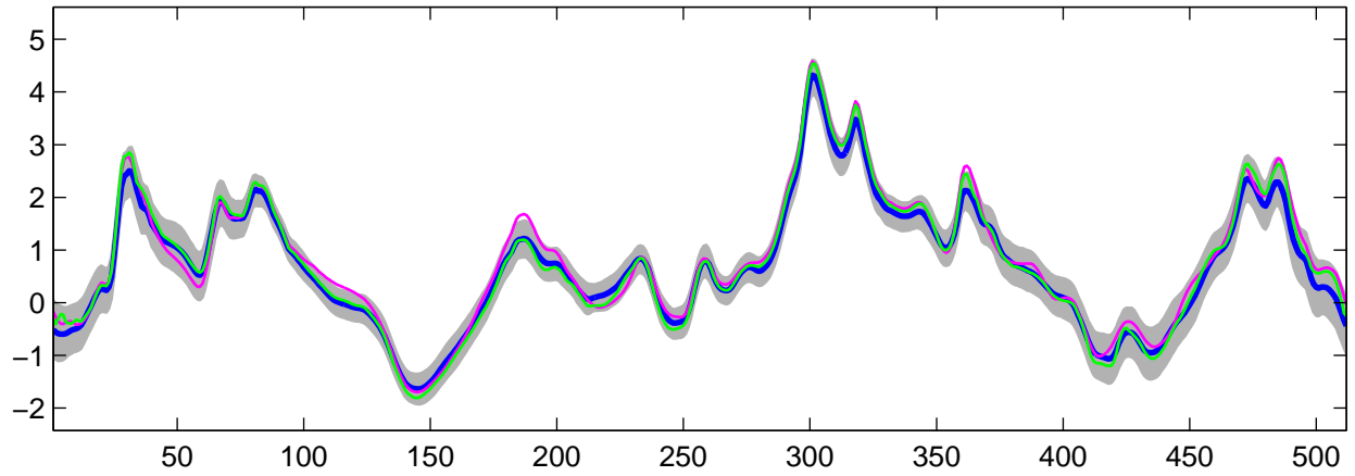
Estimated C_0(t) using G-WFMM: DE data, run 10
