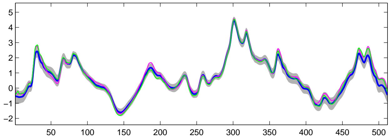
Estimated C_0(t) using R-WFMM: DE data, run 10
