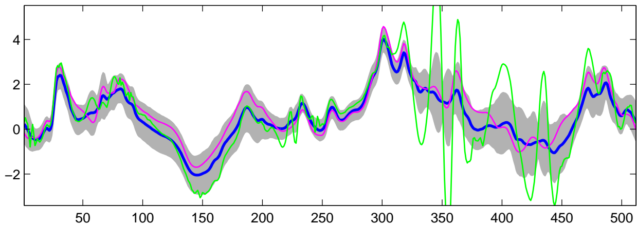
Estimated C_0(t) using G-WFMM: t_1 data, run 10
