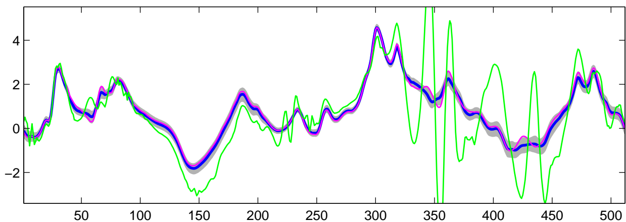
Estimated C_0(t) using R-WFMM: t_1 data, run 10
