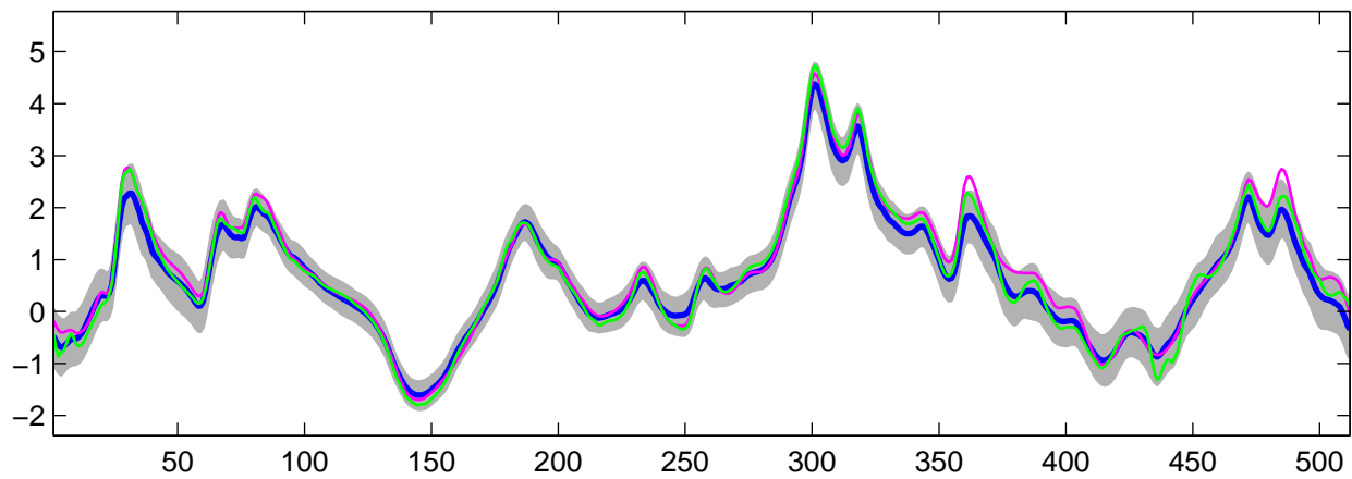
Estimated C_0(t) using G-WFMM: t_2 data, run 10
