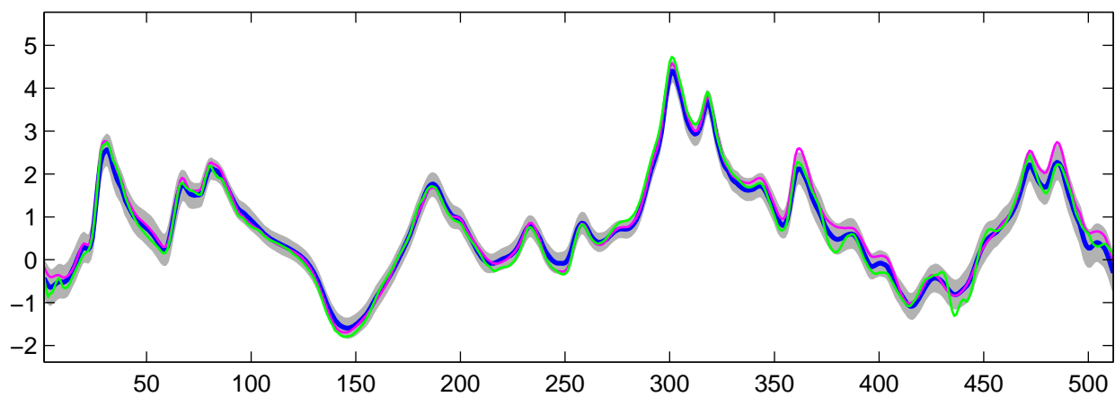
Estimated C_0(t) using R-WFMM: t_2 data, run 10
