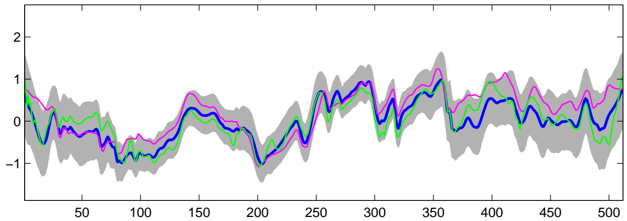
Estimated C_1(t) using R-WFMM: DE data, run 10
