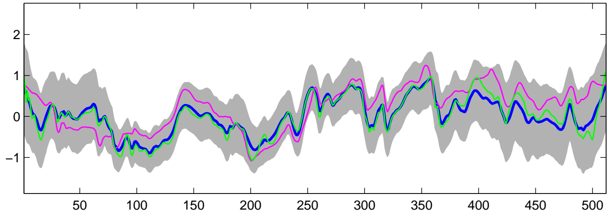
Estimated C_1(t) using G-WFMM: DE data, run 10
