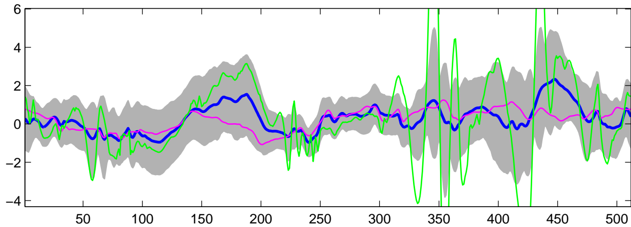
Estimated C_1(t) using G-WFMM: t_1 data, run 10
