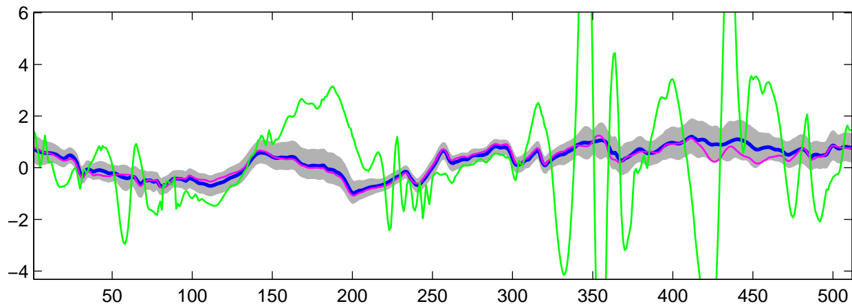
Estimated C_1(t) using R-WFMM: t_1 data, run 10
