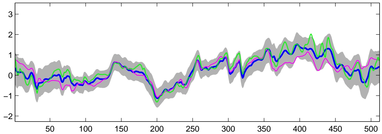
Estimated C_1(t) using R-WFMM: t_2 data, run 10
