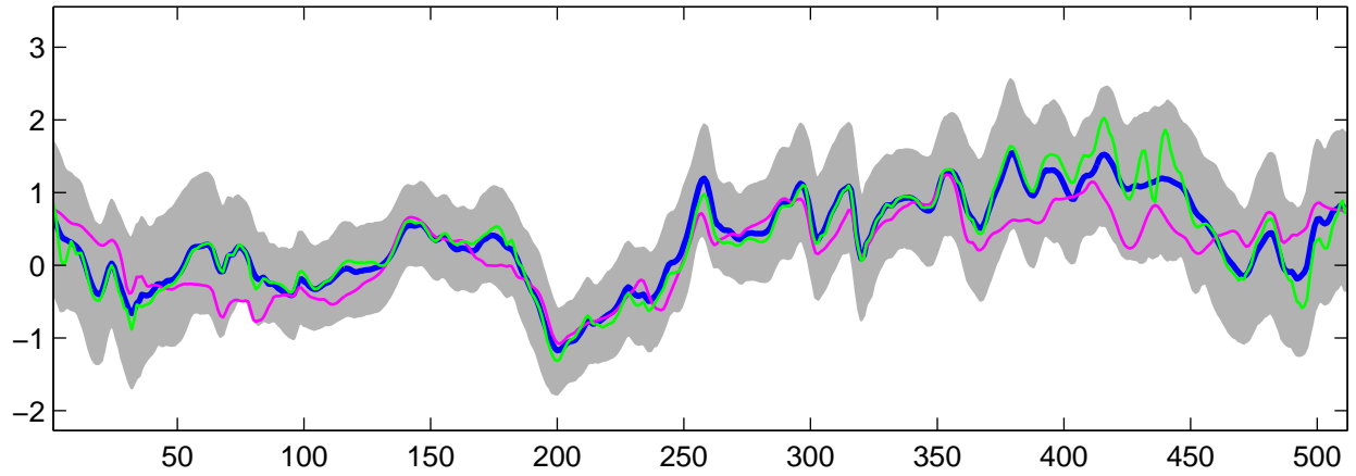
Estimated C_1(t) using G-WFMM: t_2 data, run 10
