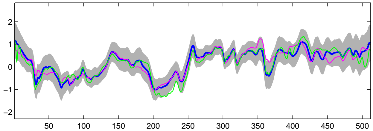
Estimated C_1(t) using R-WFMM: t_3 data, run 10
