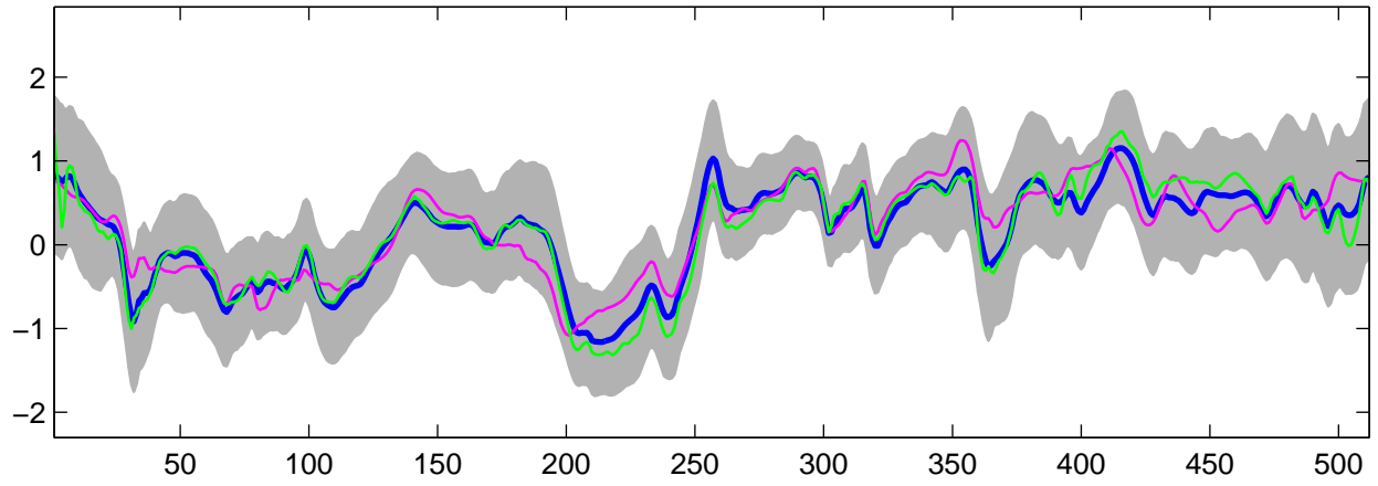
Estimated C_1(t) using G-WFMM: t_3 data, run 10
