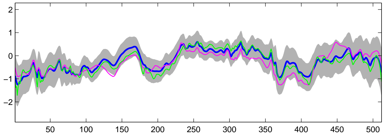
Estimated C_2(t) using R-WFMM: DE data, run 10
