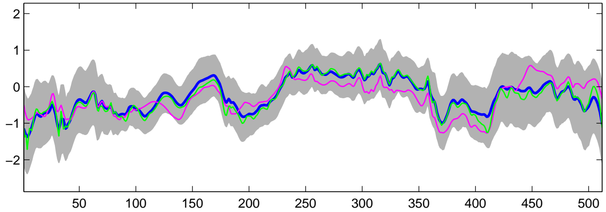
Estimated C_2(t) using G-WFMM: DE data, run 10
