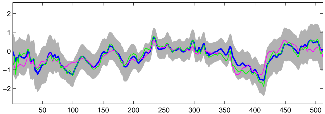
Estimated C_2(t) using R-WFMM: Normal data, run 10
