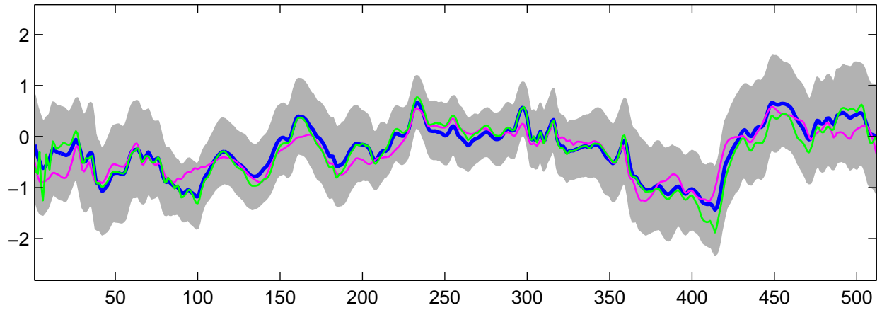
Estimated C_2(t) using G-WFMM: Normal data, run 10
