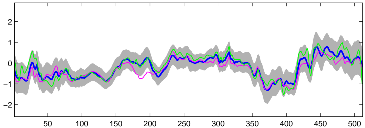
Estimated C_2(t) using R-WFMM: t_2 data, run 10
