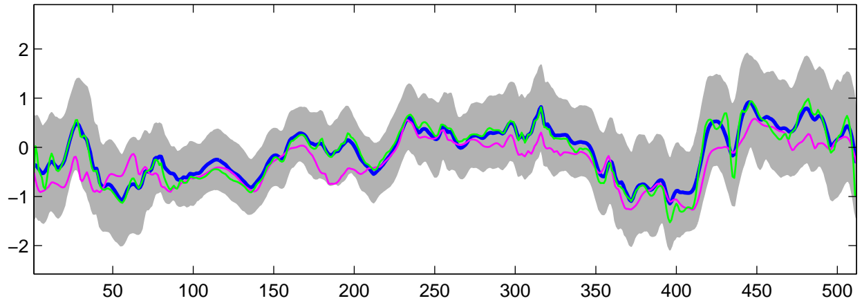
Estimated C_2(t) using G-WFMM: t_2 data, run 10
