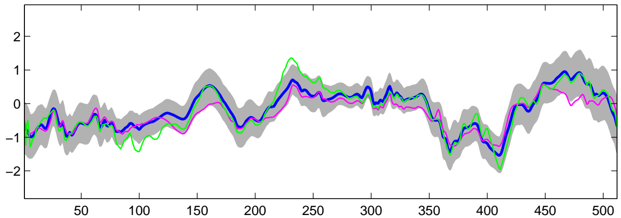
Estimated C_2(t) using R-WFMM: t_3 data, run 10
