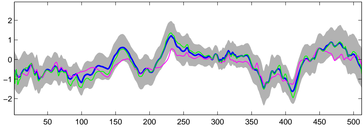
Estimated C_2(t) using G-WFMM: t_3 data, run 10
