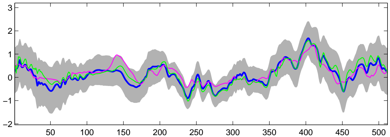
Estimated C_3(t) using R-WFMM: Normal data, run 10
