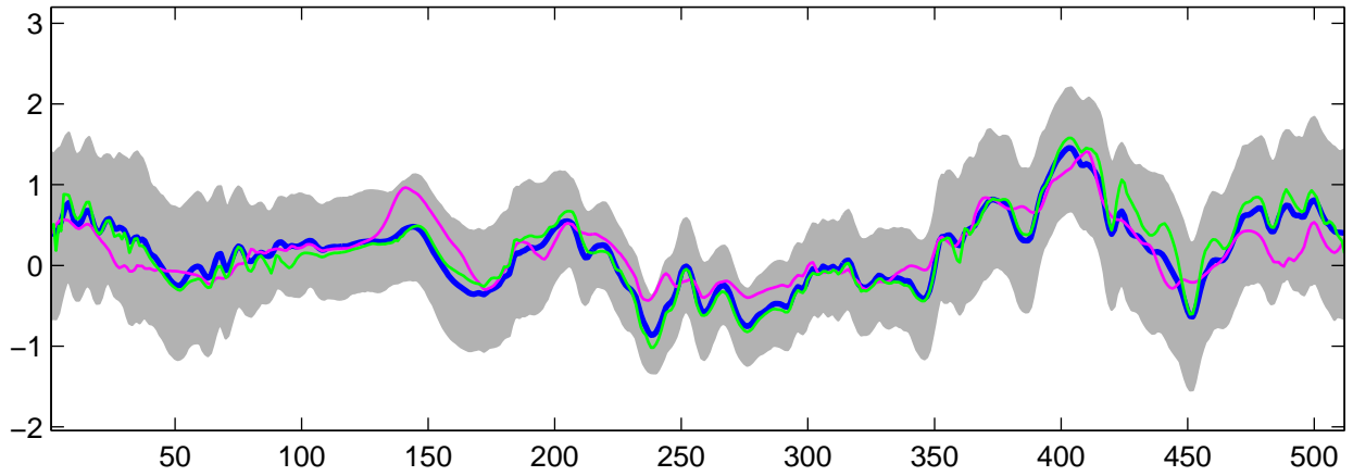
Estimated C_3(t) using G-WFMM: Normal data, run 10
