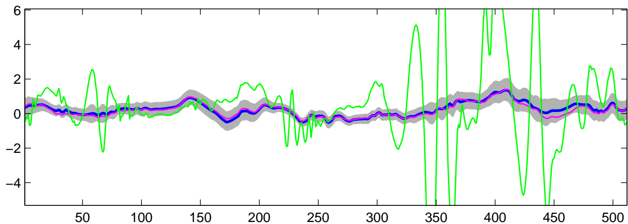
Estimated C_3(t) using R-WFMM: t_1 data, run 10
