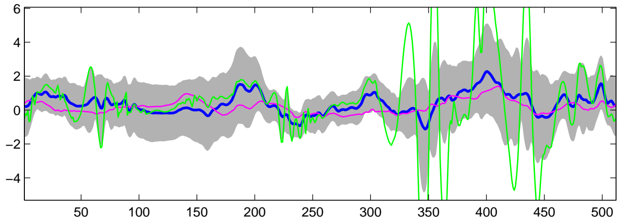
Estimated C_3(t) using G-WFMM: t_1 data, run 10
