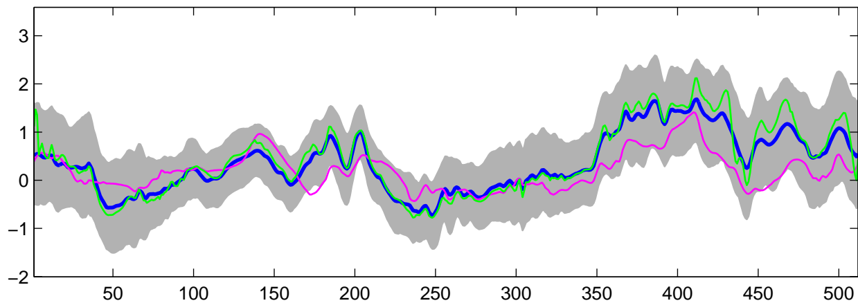
Estimated C_3(t) using G-WFMM: t_2 data, run 10
