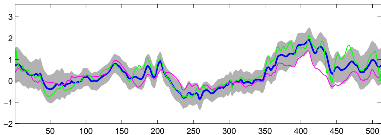
Estimated C_3(t) using R-WFMM: t_2 data, run 10
