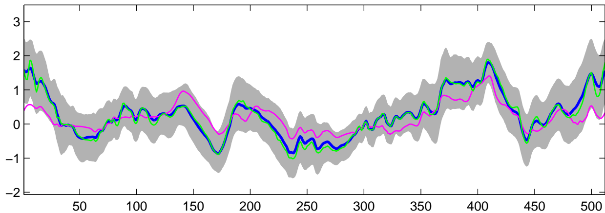
Estimated C_3(t) using G-WFMM: t_3 data, run 10
