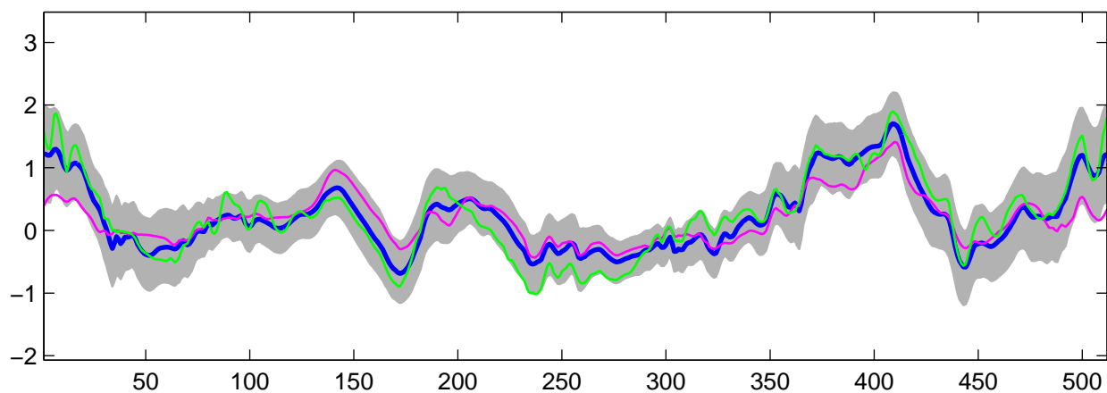
Estimated C_3(t) using R-WFMM: t_3 data, run 10
