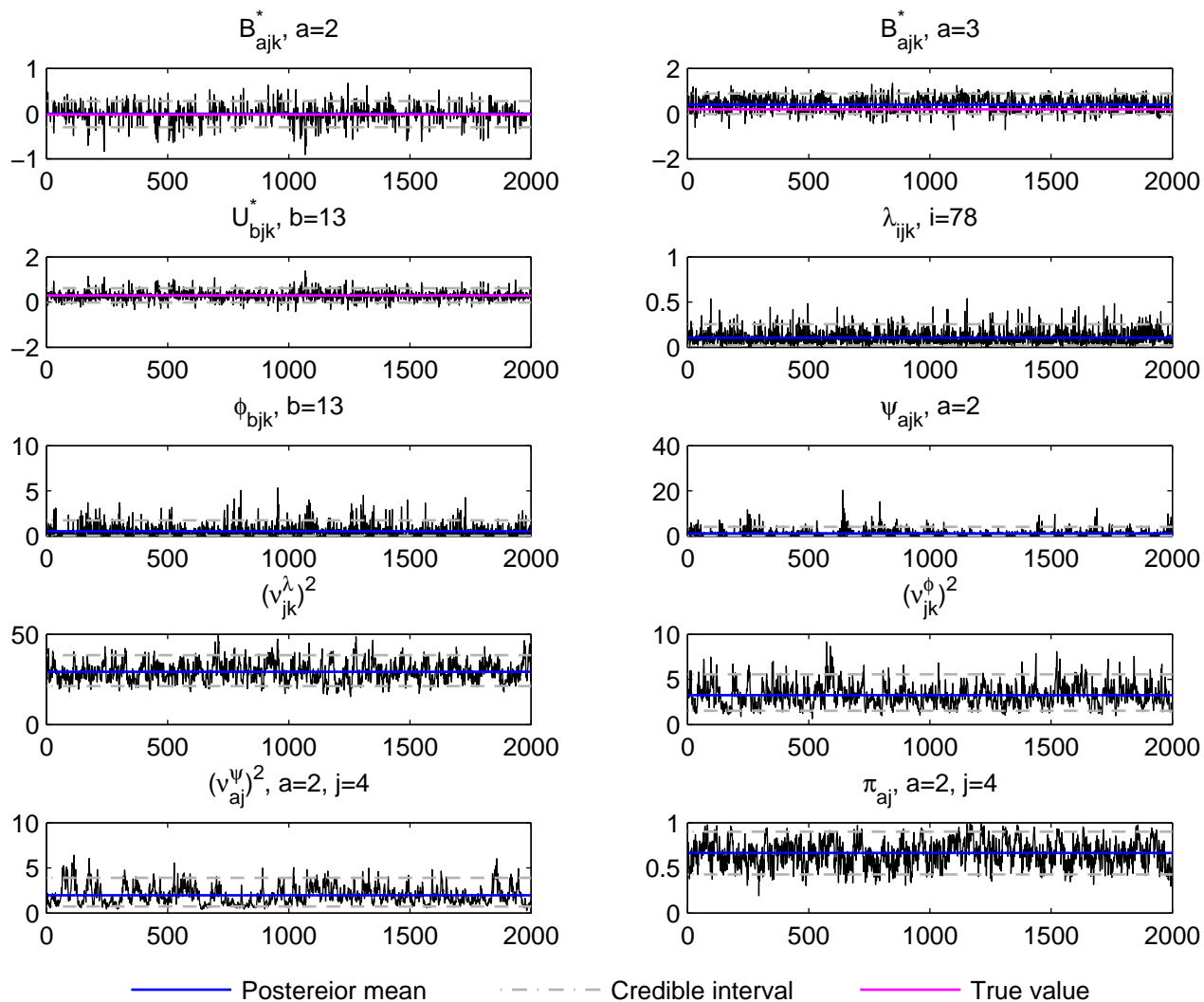
Trace plot, j=4, k=6 , DE data, simulation run 10
