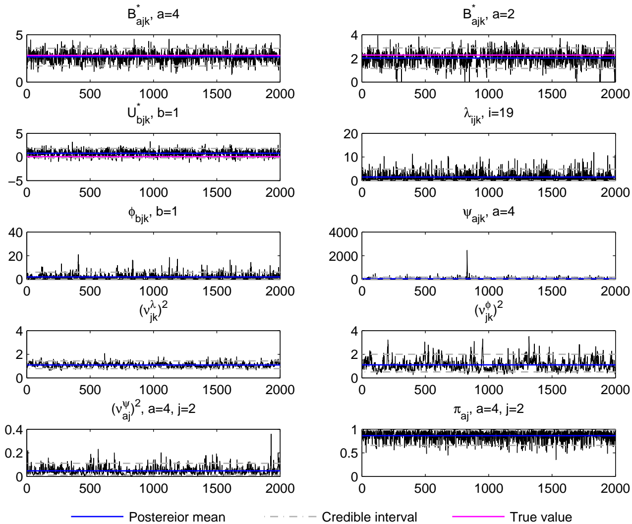
Trace plot, j=2, k=6 , Normal data, simulation run 10
