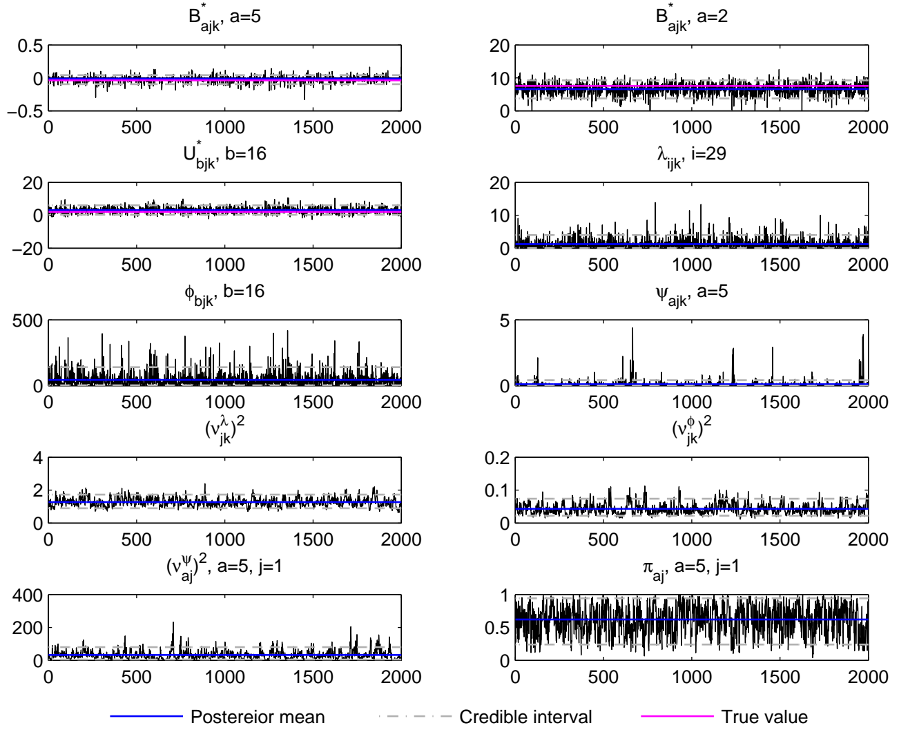
Trace plot, j=1, k=4, t_1 data, simulation run 10
