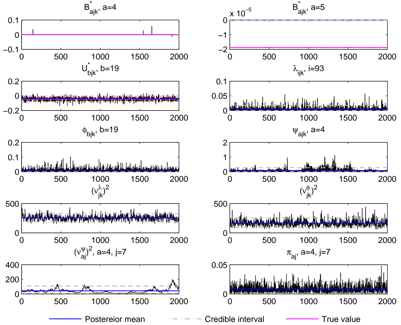
Trace plot, j=7, k=1, t_2 data, simulation run 10
