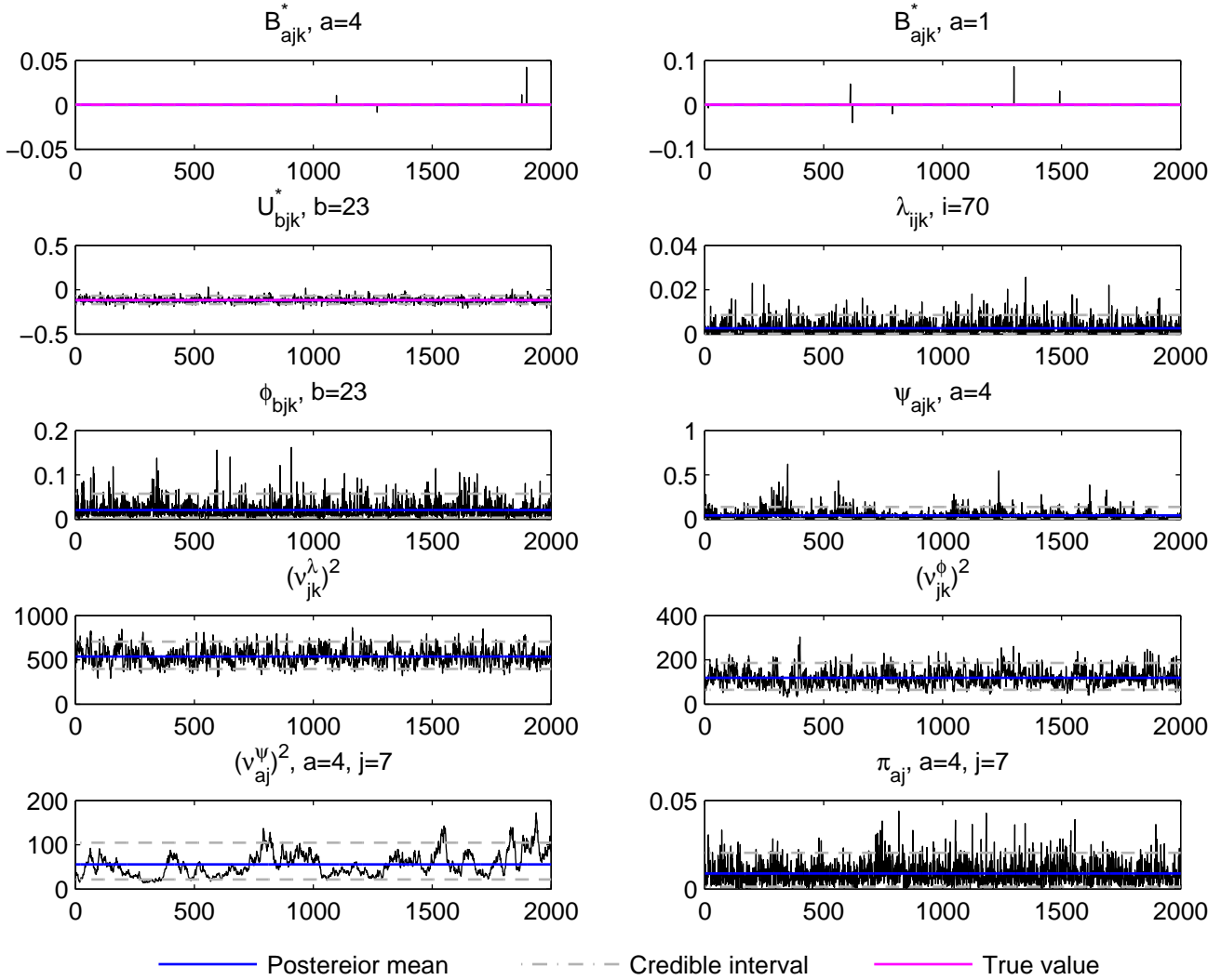
Trace plot, j=7, k=1, t_3 data, simulation run 10
