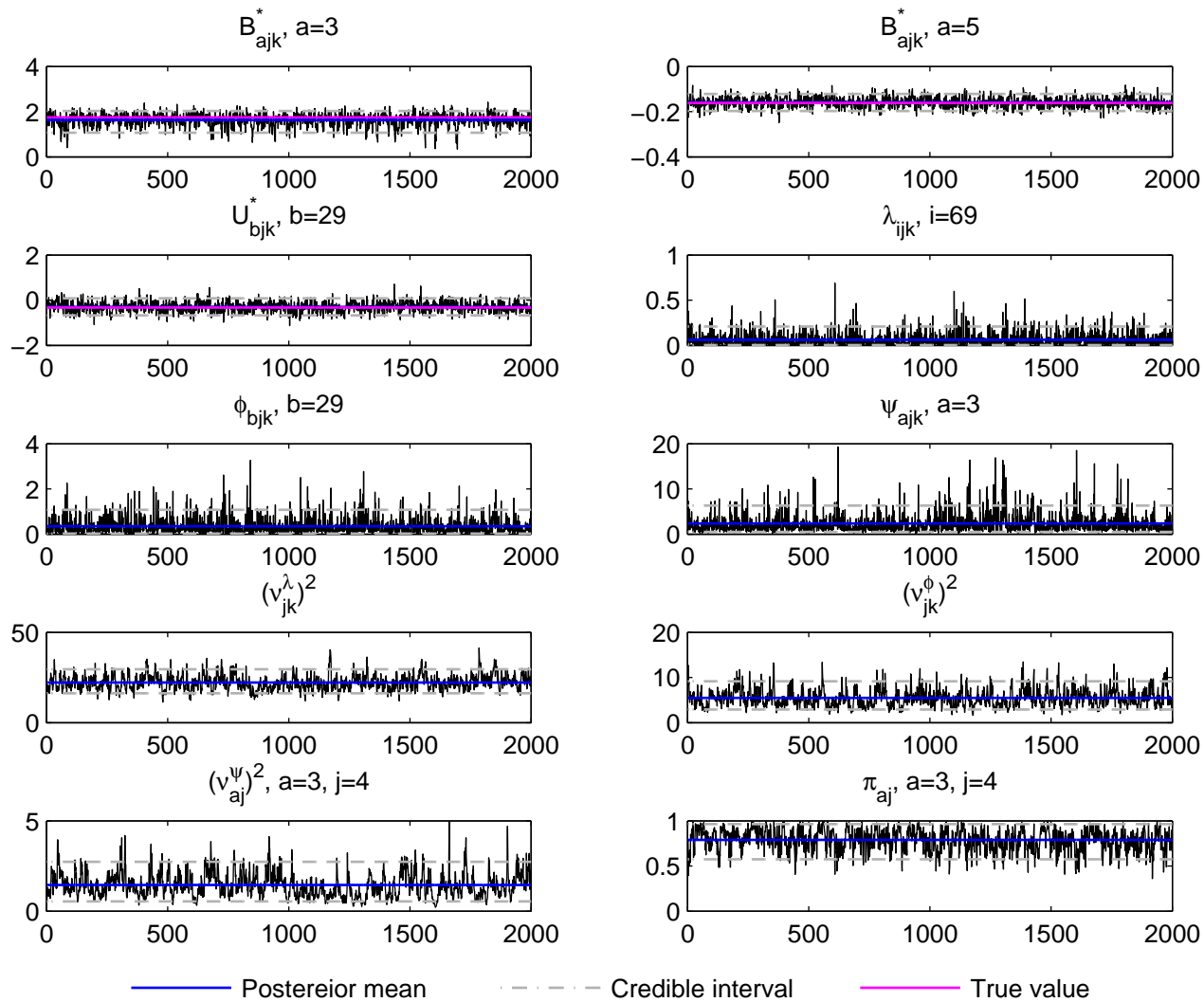
Trace plot, j=4, k=3 , DE data, simulation run 10
