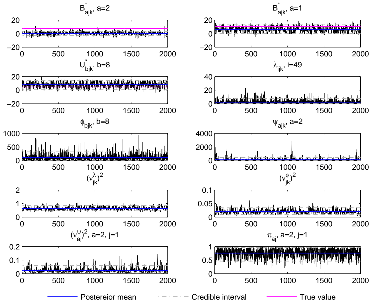
Trace plot, j=1, k=4 , Normal data, simulation run 10
