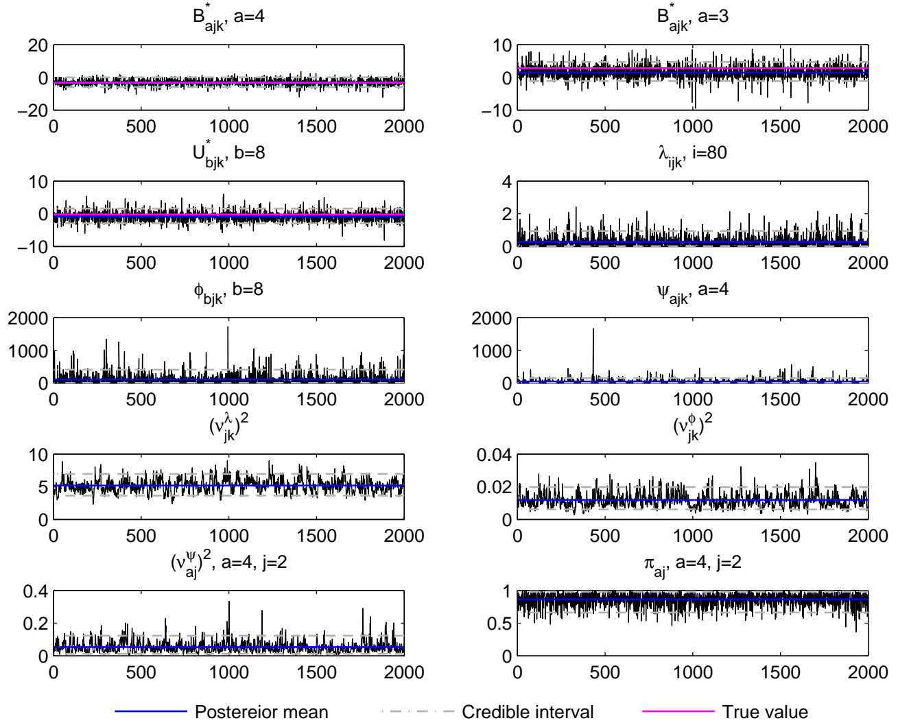
Trace plot, j=2, k=7, t_1 data, simulation run 10
