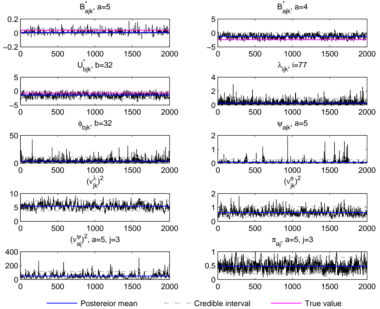
Trace plot, j=3, k=3, t_2 data, simulation run 10
