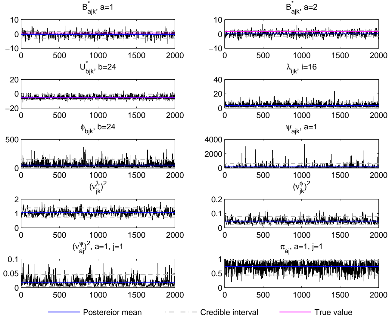
Trace plot, j=1, k=7, t_3 data, simulation run 10
