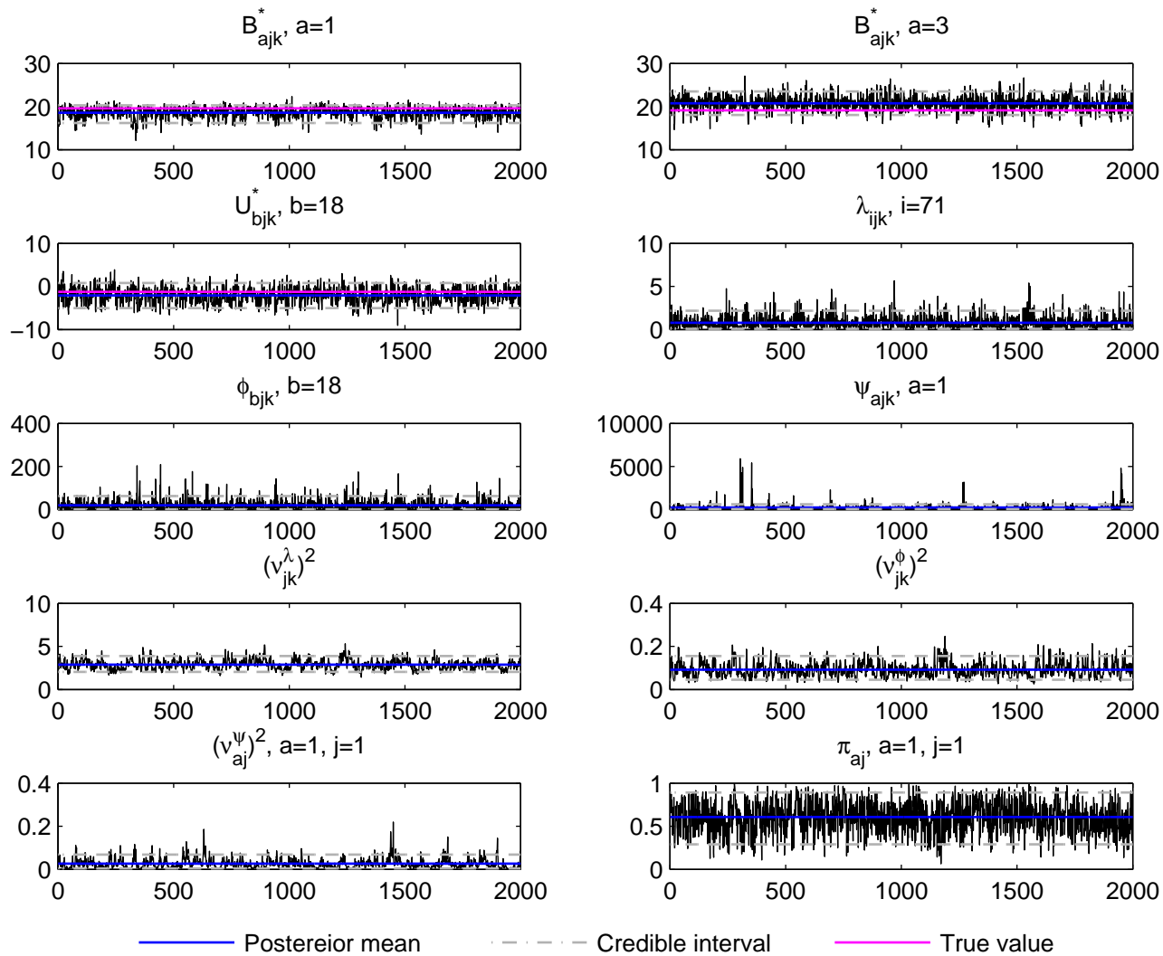
Trace plot, j=1, k=1 , DE data, simulation run 10
