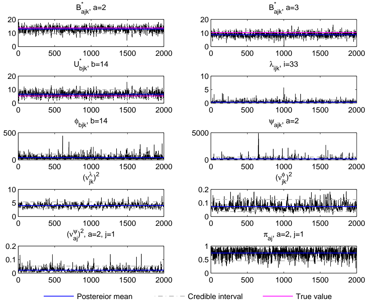
Trace plot, j=1, k=5, t_3 data, simulation run 10
