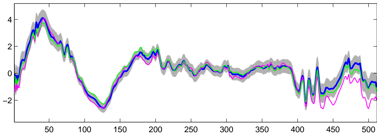
Estimated U_{10}(t) using R-WFMM: DE data, run 10
