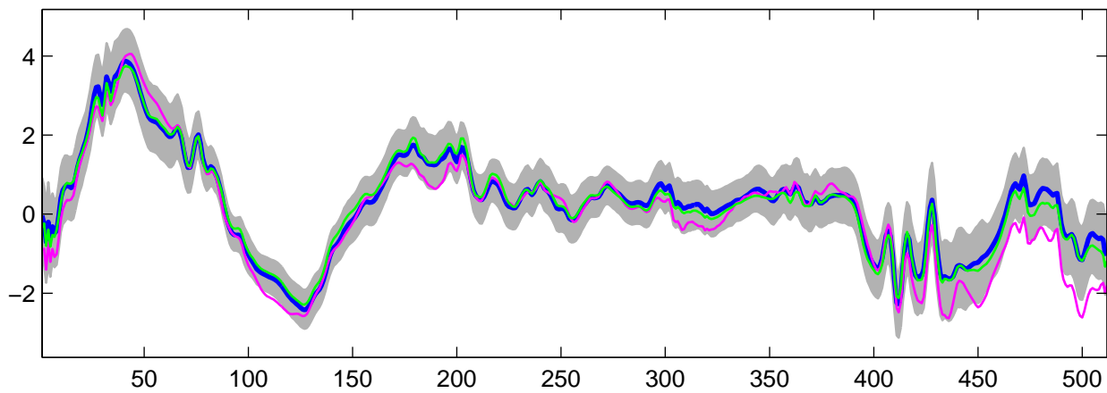
Estimated U_{10}(t) using G-WFMM: DE data, run 10
