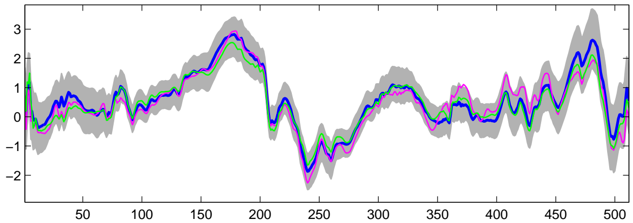
Estimated U_{10}(t) using R-WFMM: Normal data, run 10
