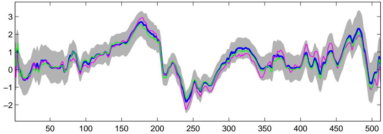
Estimated U_{10}(t) using G-WFMM: Normal data, run 10
