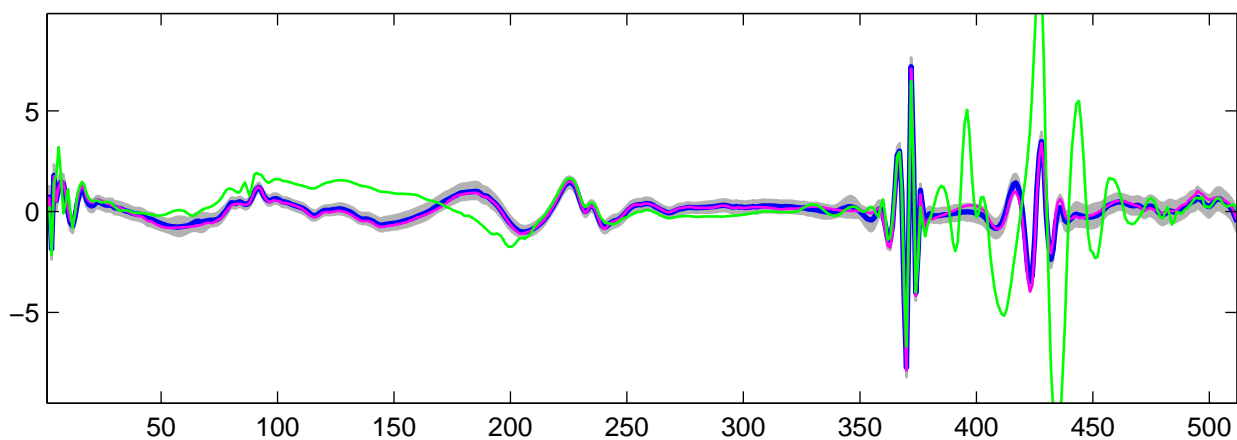
Estimated U_{10}(t) using R-WFMM: t_1 data, run 10
