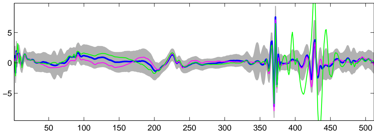
Estimated U_{10}(t) using G-WFMM: t_1 data, run 10
