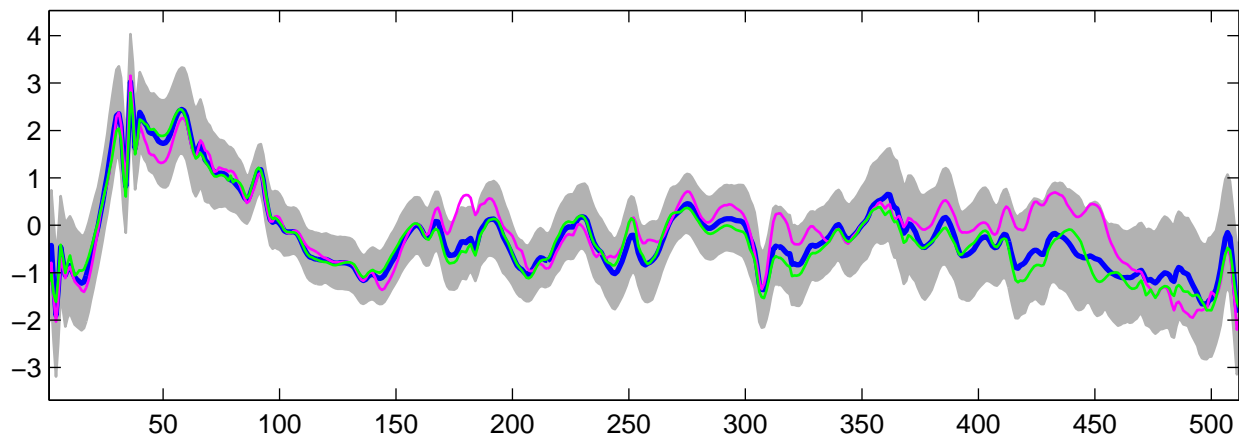
Estimated U_{10}(t) using G-WFMM: t_2 data, run 10
