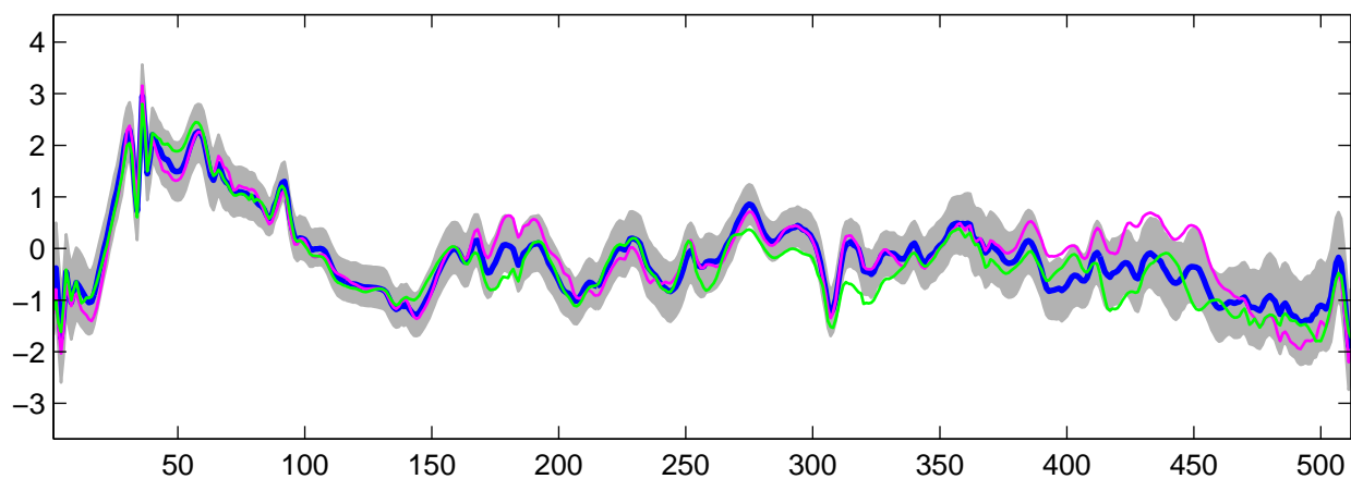
Estimated U_{10}(t) using R-WFMM: t_2 data, run 10
