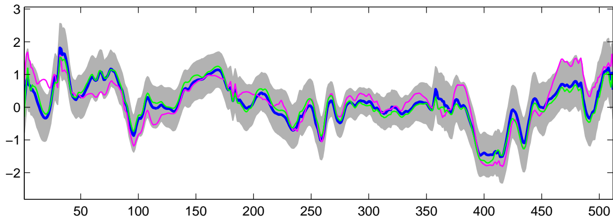
Estimated U_{10}(t) using G-WFMM: t_3 data, run 10
