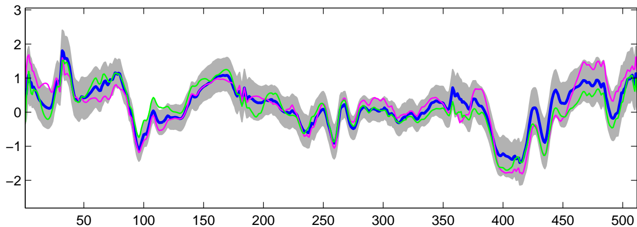
Estimated U_{10}(t) using R-WFMM: t_3 data, run 10
