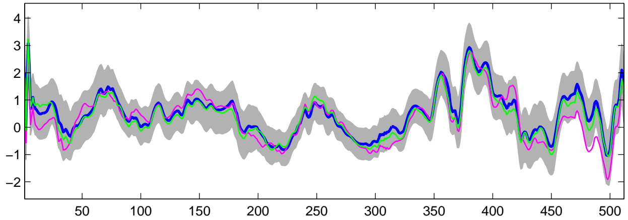
Estimated U_{11}(t) using G-WFMM: Normal data, run 10
