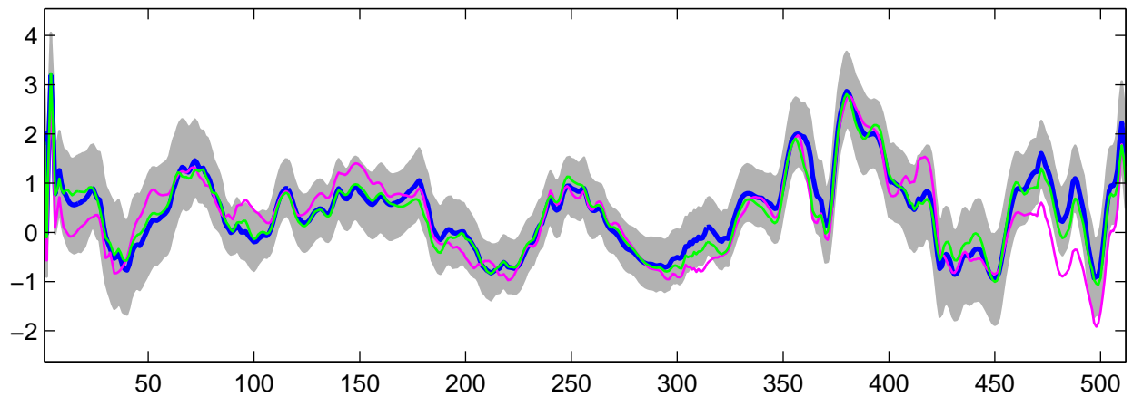
Estimated U_{11}(t) using R-WFMM: Normal data, run 10
