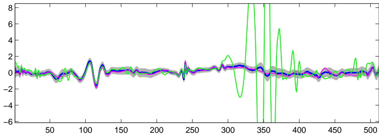
Estimated U_{11}(t) using R-WFMM: t_1 data, run 10
