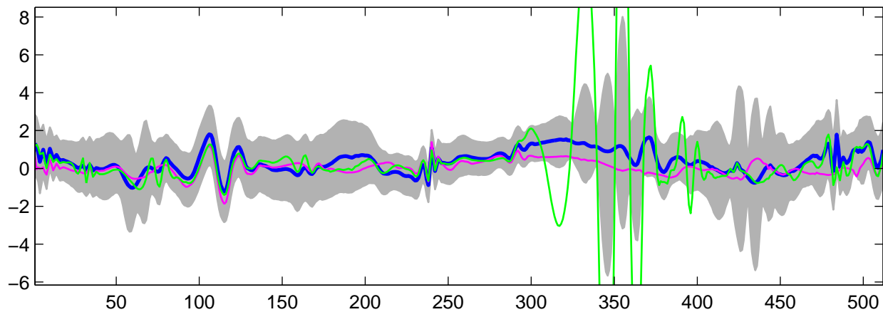
Estimated U_{11}(t) using G-WFMM: t_1 data, run 10
