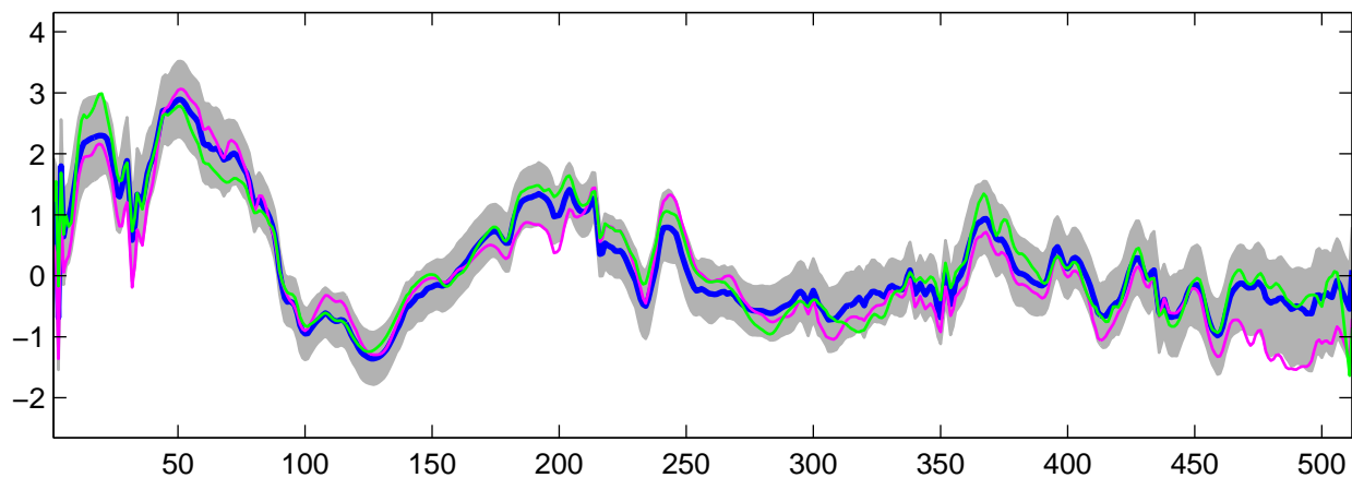
Estimated U_{11}(t) using R-WFMM: t_2 data, run 10
