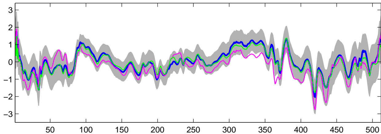
Estimated U_{12}(t) using G-WFMM: DE data, run 10
