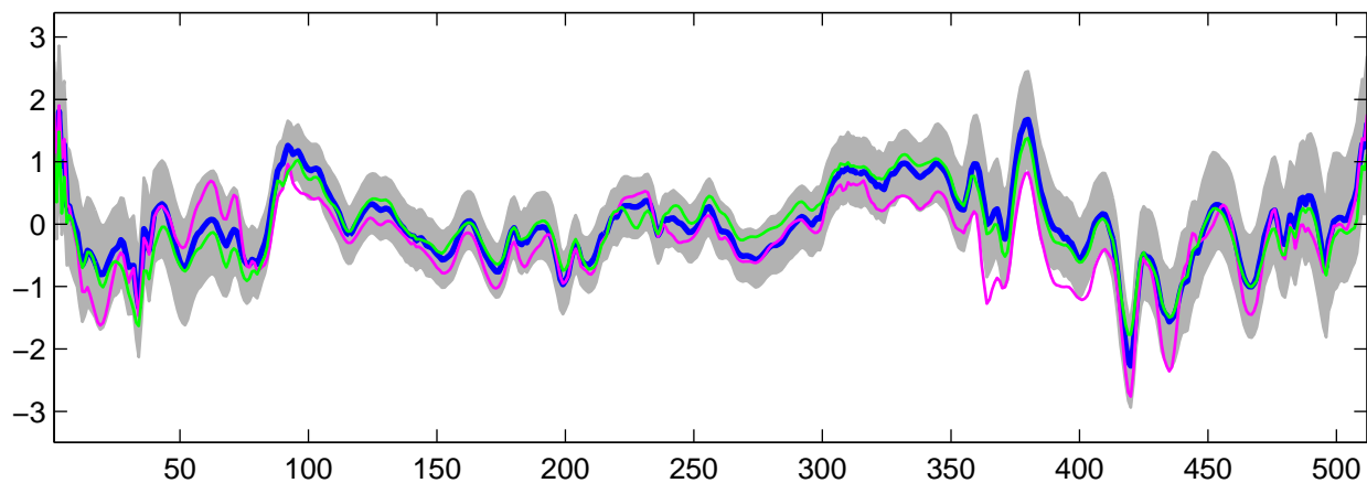
Estimated U_{12}(t) using R-WFMM: DE data, run 10
