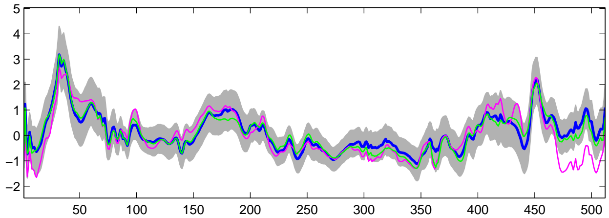
Estimated U_{12}(t) using R-WFMM: Normal data, run 10
