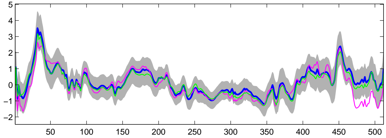
Estimated U_{12}(t) using G-WFMM: Normal data, run 10
