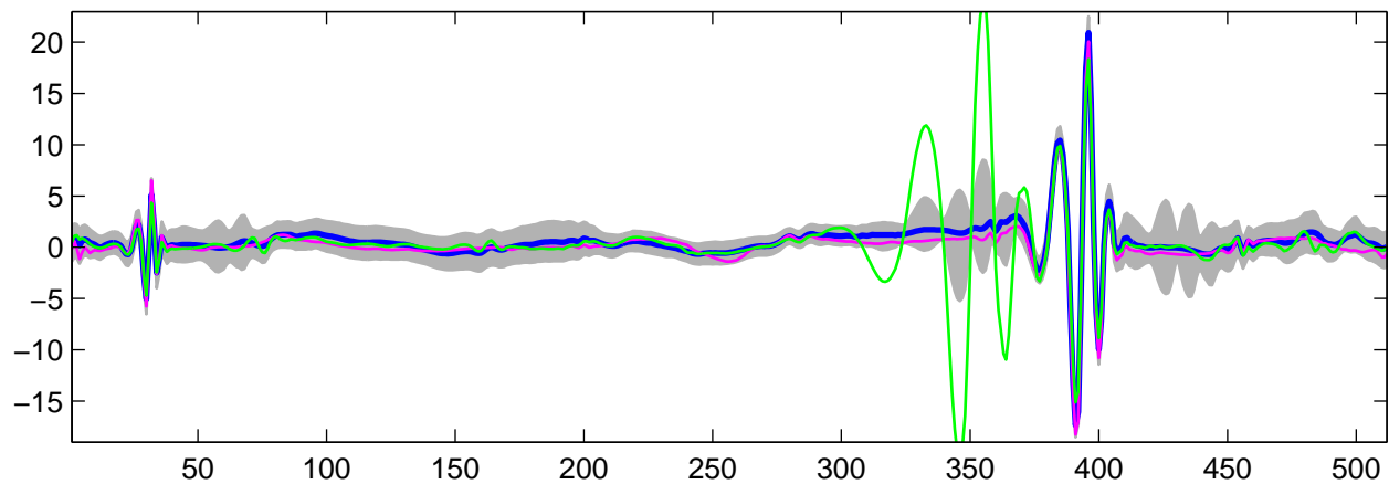
Estimated U_{12}(t) using G-WFMM: t_1 data, run 10
