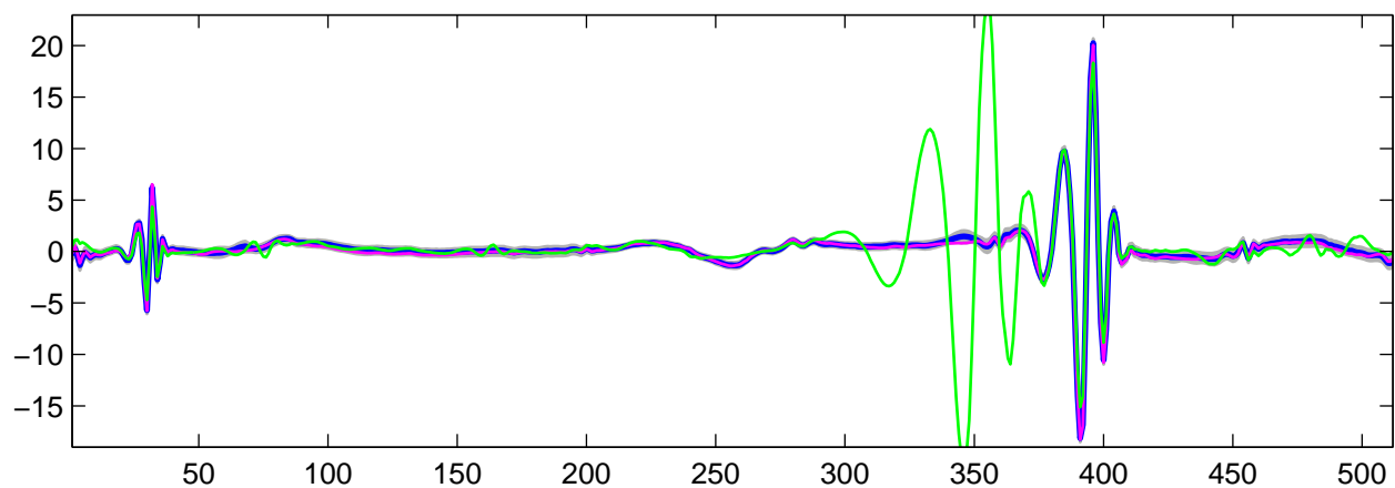
Estimated U_{12}(t) using R-WFMM: t_1 data, run 10
