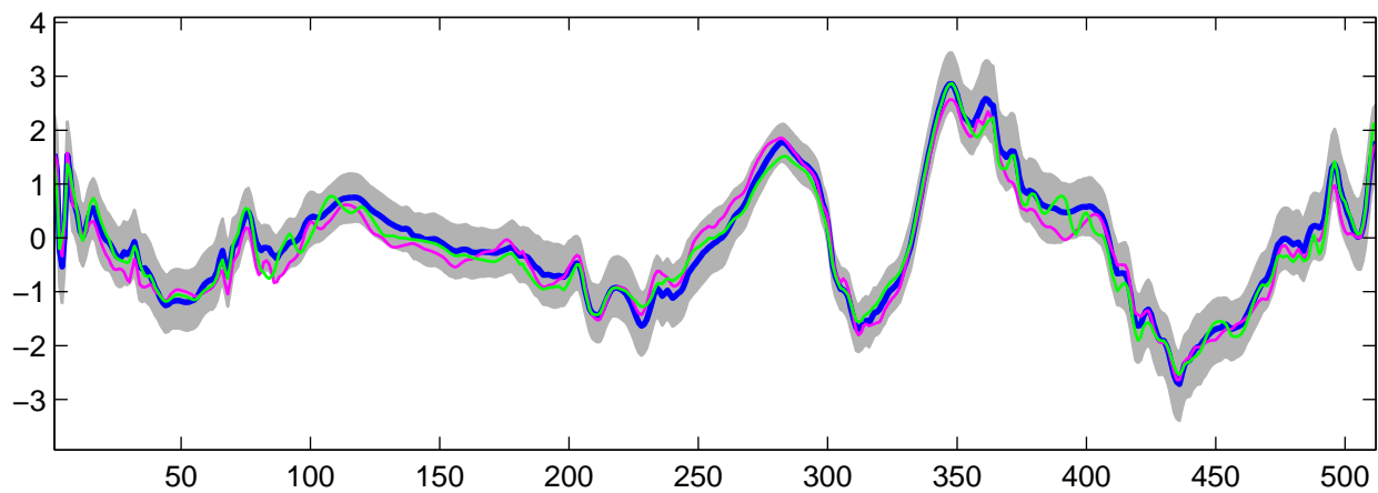
Estimated U_{12}(t) using R-WFMM: t_3 data, run 10
