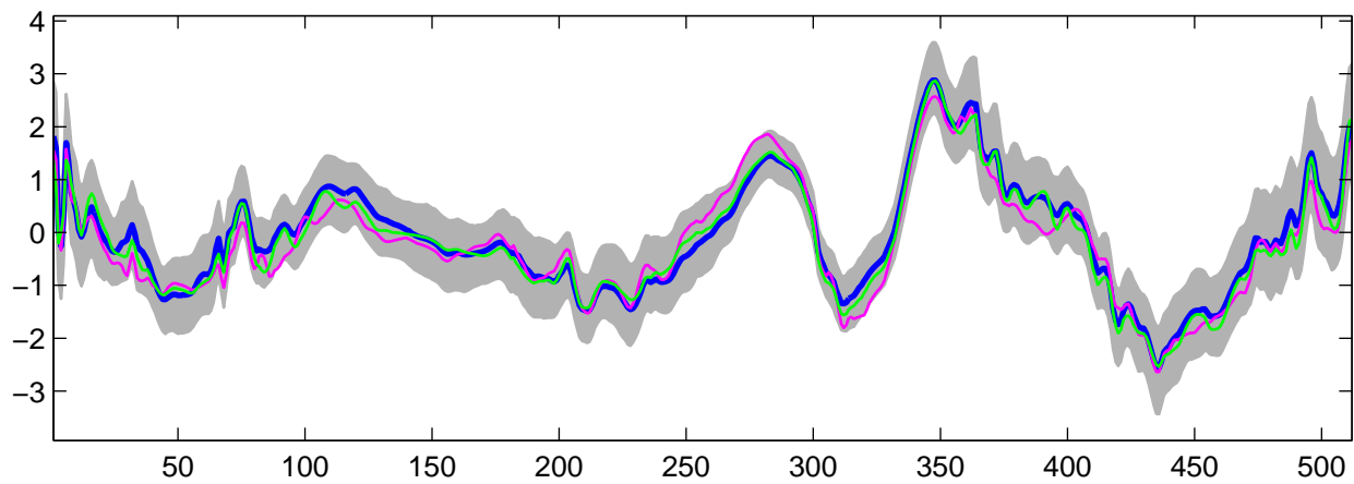
Estimated U_{12}(t) using G-WFMM: t_3 data, run 10
