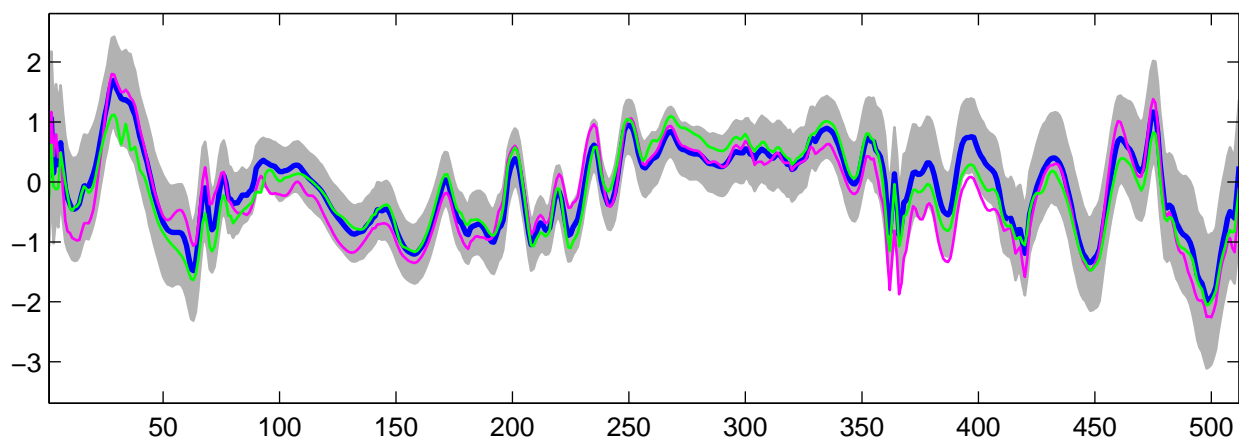
Estimated U_{13}(t) using R-WFMM: DE data, run 10
