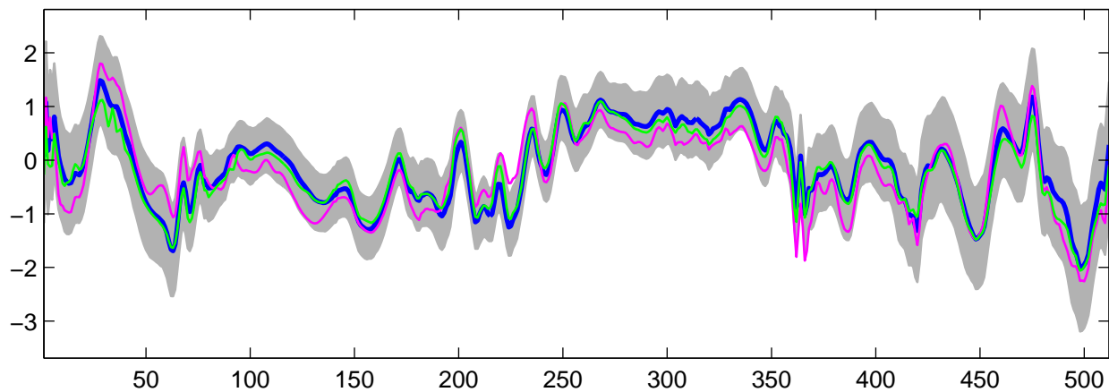
Estimated U_{13}(t) using G-WFMM: DE data, run 10
