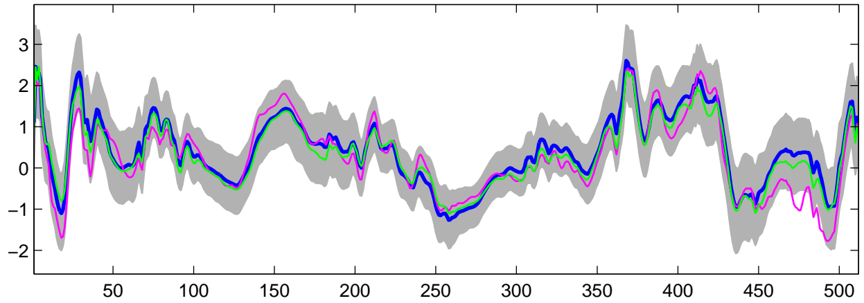
Estimated U_{13}(t) using G-WFMM: Normal data, run 10
