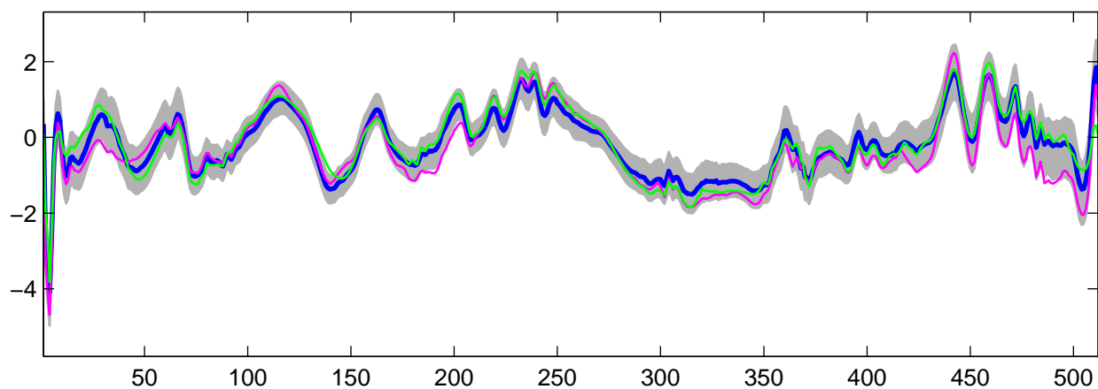
Estimated U_{13}(t) using R-WFMM: t_2 data, run 10
