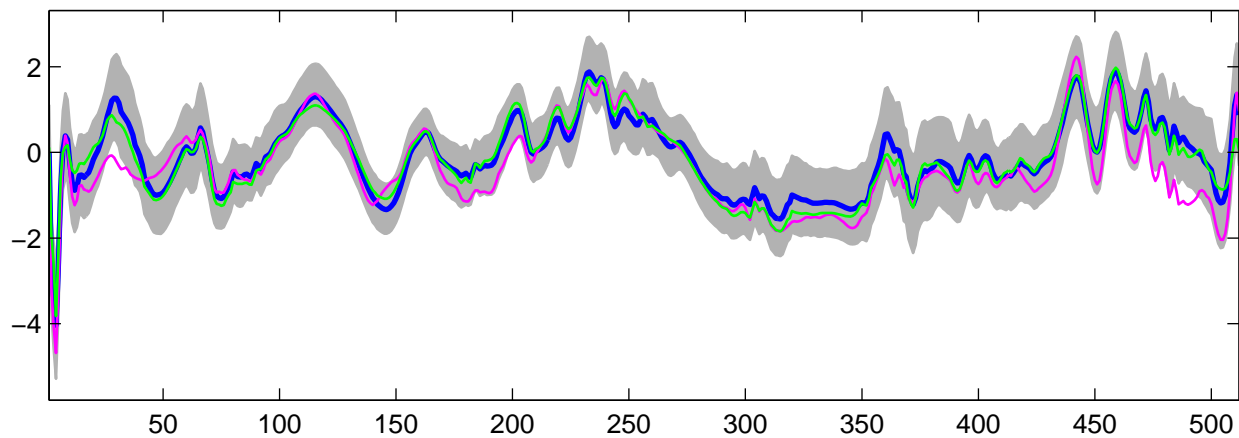
Estimated U_{13}(t) using G-WFMM: t_2 data, run 10
