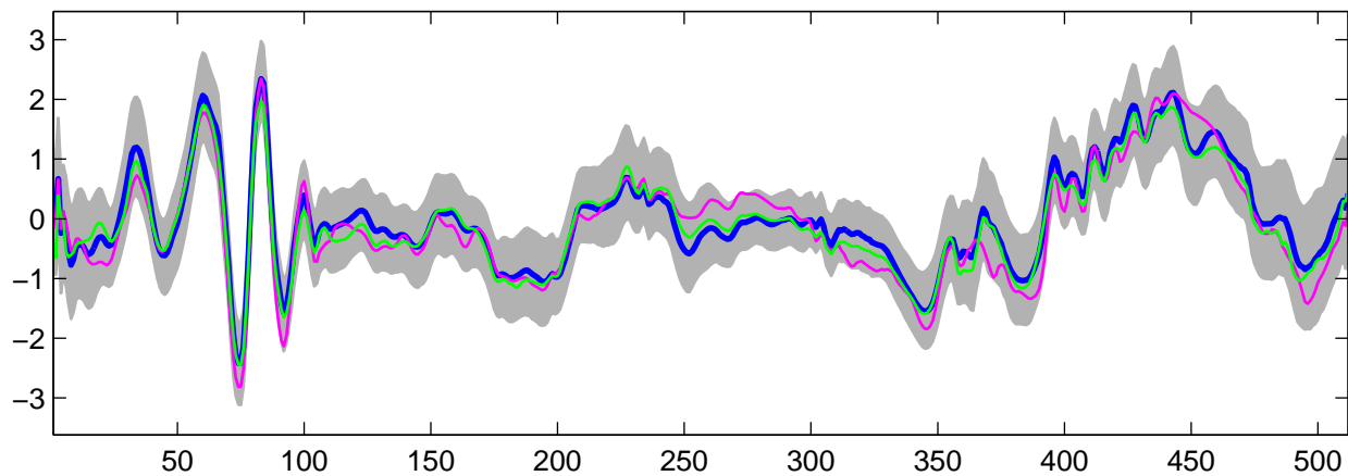
Estimated U_{13}(t) using G-WFMM: t_3 data, run 10
