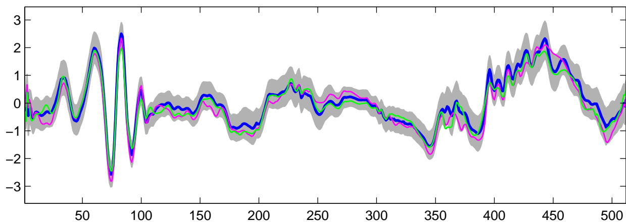
Estimated U_{13}(t) using R-WFMM: t_3 data, run 10
